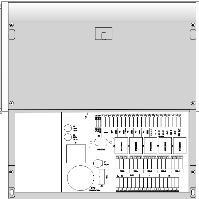
Terminal box
